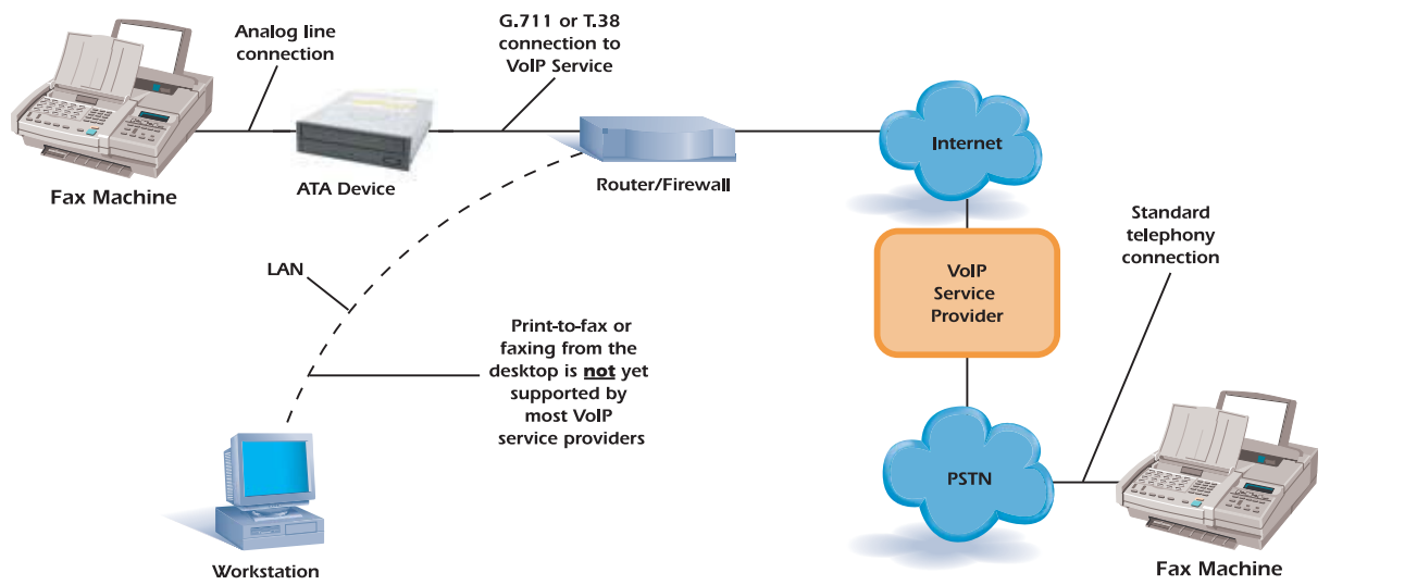
Figure 4 VoIP Service Provider (fax support through fax machines connected to ATA devices)
